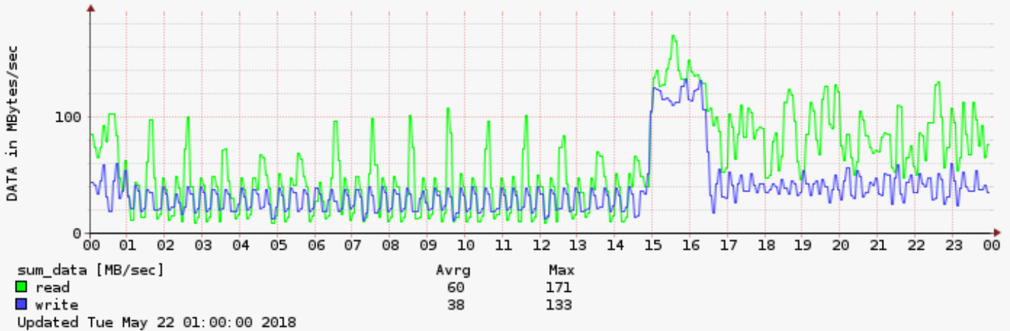
Fujitsu-ETERNUS-AF-DX : POOL : aggregated: resp_t : 00:00:00 20.05.2018 - 00:00:00 21.05.2018
